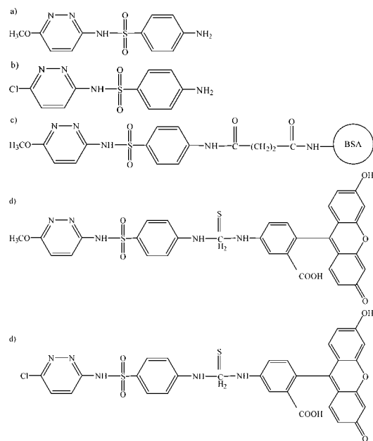
Figure 1. Chemical structures of sulfonamides (a) SMP and (b) SCP, (c) immunogen, and tracers (d) SMP-FITC and (e) SCP-FITC.
