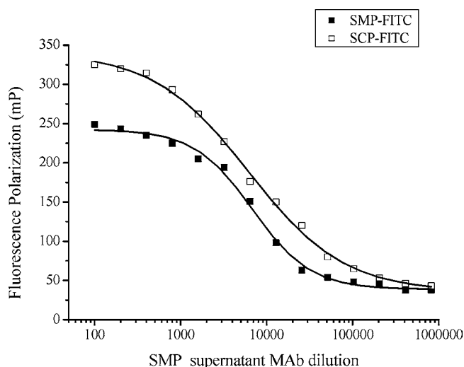
Figure 2. Dilution curves for SMP monoclonal antibody with different tracers SMP-FITC and SCP-FITC.
