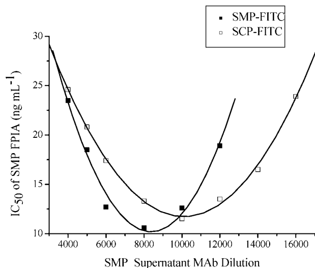
Figure 3. Relationship curve between IC_{50} and antibody dilution.
