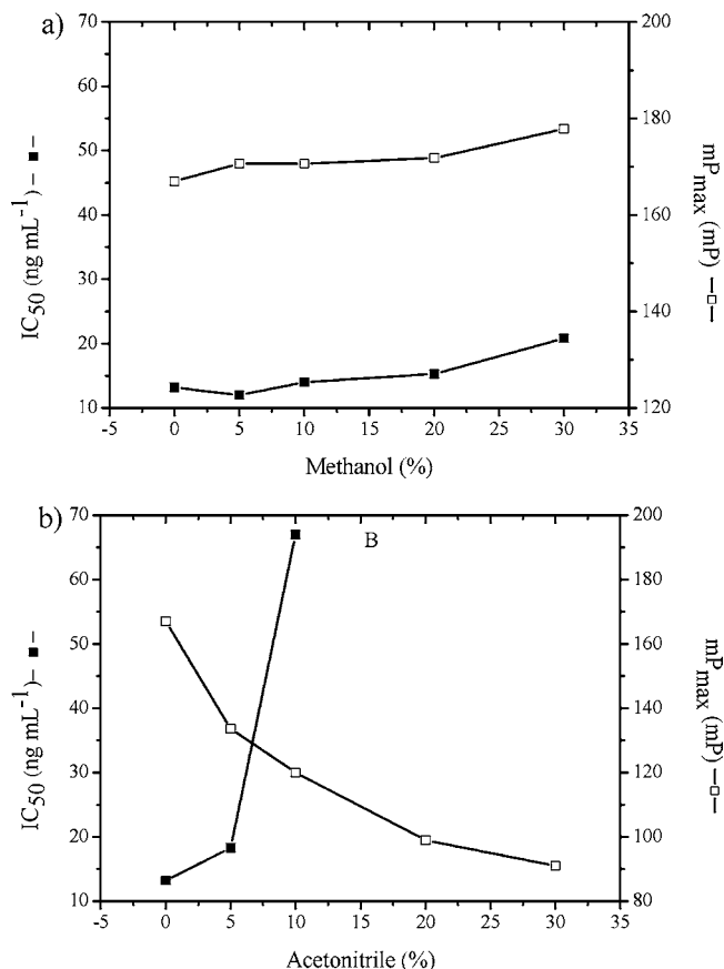
Figure 6. Effect of (a) methanol and (b) acetonitrile on SMP FPIA performance: (■) value of IC_{50} for SMP and (□) mP value in the absence of SMP ( mP_{max} ). Values refer to the final concentrations of solvents (v/v) in the competitive assay solution. Each point represents the mean of three replicates.
