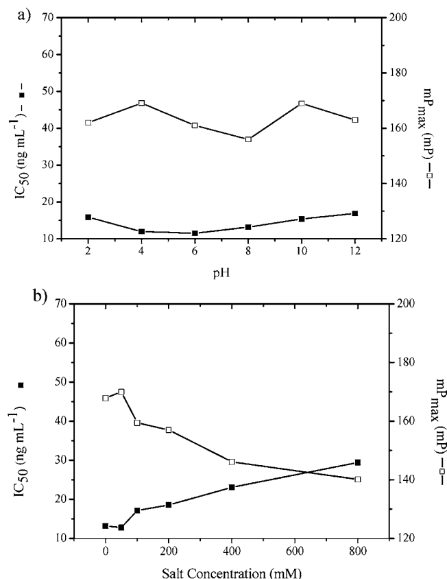
Figure 5. Influence of the (a) pH and (b) salt concentration of assay buffer on the analytical characteristics of SMP competitive standard curve: (■) value of IC_{50} for SMP and (□) mP value in the absence of SMP ( mP_{max} ). All reagents were prepared in BB at the appropriate pH and salt concentration. Each point represents the mean of three replicates.
