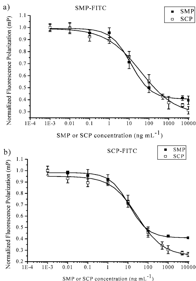
Figure 4. FPIA calibration curves for SMP and SCP using the same Mab and two different tracers: (a) SMP-FITC and (b) SCP-FITC. FPIA calibration curve and the SCP and SMP standard drug were dissolved in BB buffer. FP values, which are means of three replicates, were plotted against analyte concentration.
