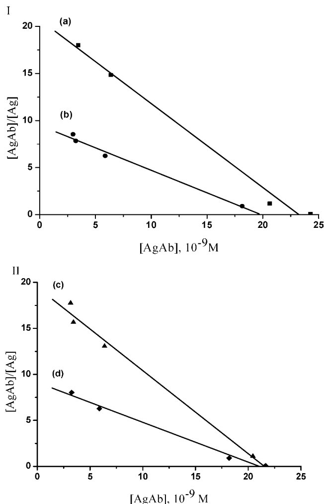
Figure 7. Scatchard plot for K_{aff} calculation. I: (a) tracer SCP-FITC, antigen SMP, Y = -0.903X + 19.442 ; (b) tracer SCP-FITC, antigen SCP, Y = -0.433X + 9.121 . II: (c) tracer SMP-FITC, antigen SMP, Y = -0.891X + 20.716 ; (d) tracer SMP-FITC, antigen SCP, Y = -0.478X + 9.488 .
